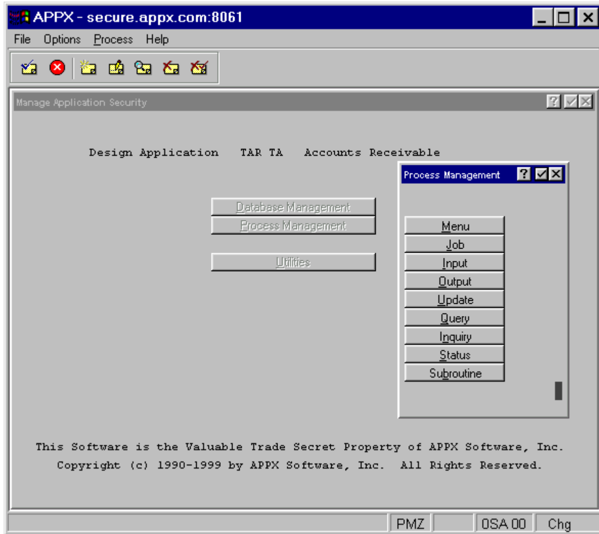
Figure 5-7. Process Security Management Overlay
