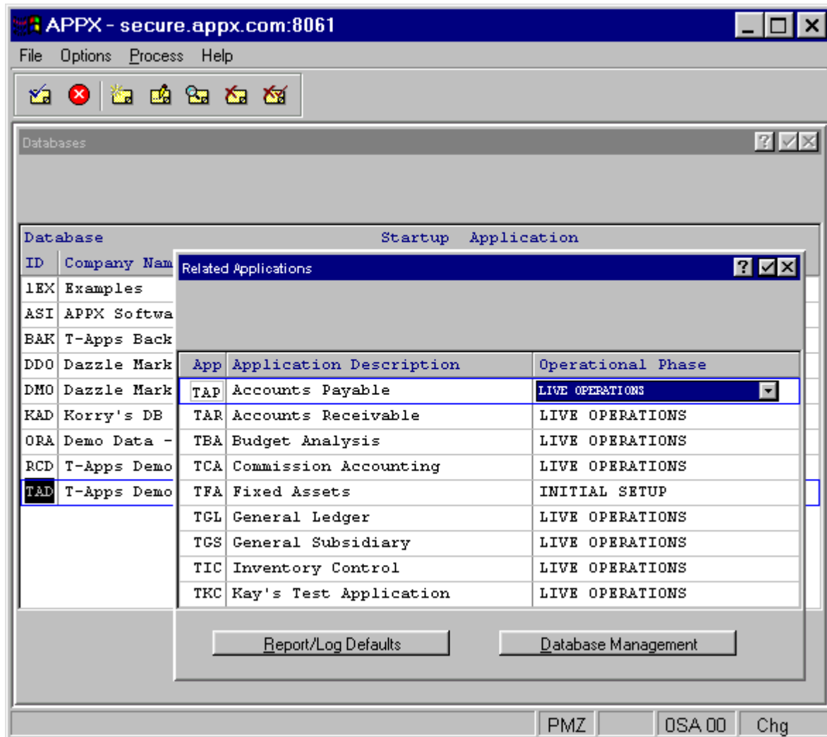
Figure 2-33. Databases Related Applications Overlay
