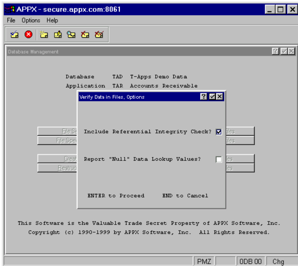
Figure 3-13. Verify Data In Files Options Overlay
