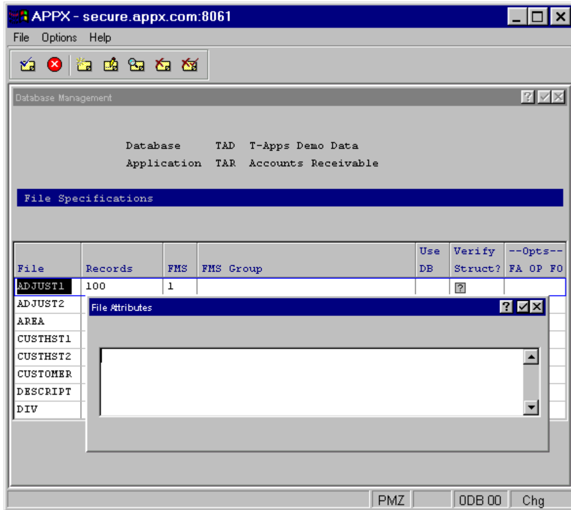
Figure 3-4. File Attributes Overlay for ISAM (Types 1,2,3)
