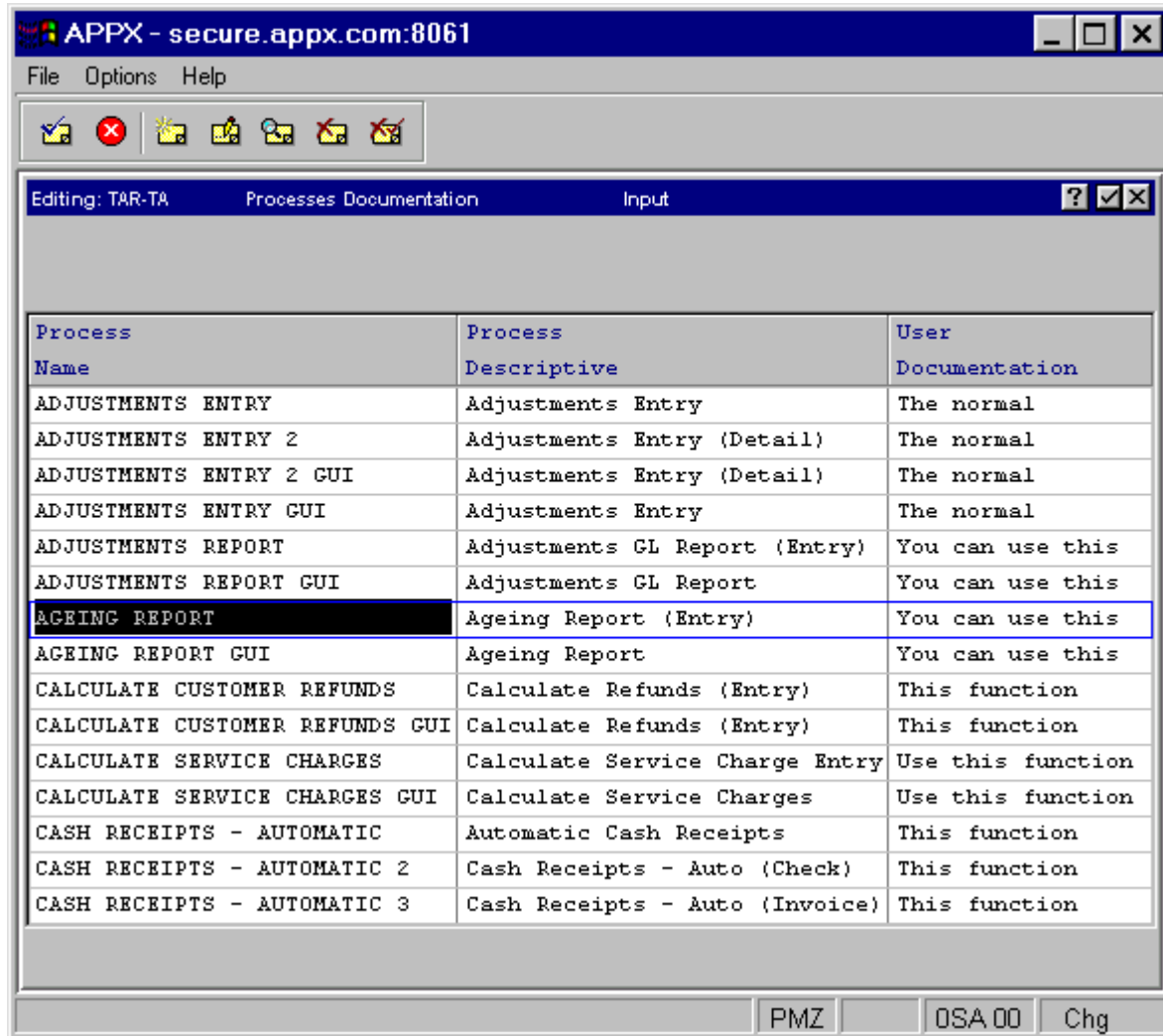
Figure 4-9. Select Process Documentation Screen (for Input Processes)
