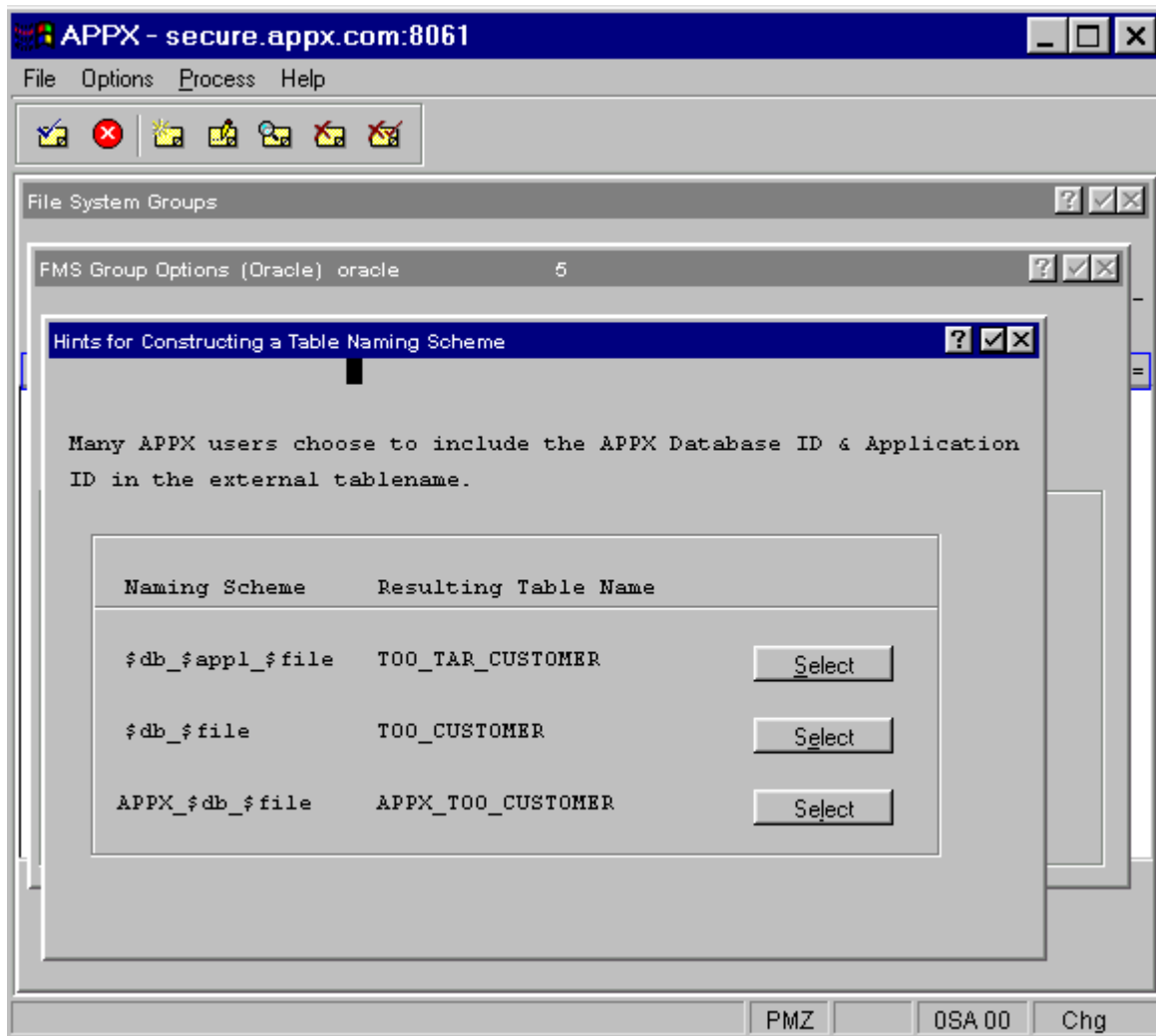
Figure 2-20-A. Table Naming Scheme Hints Overlay
