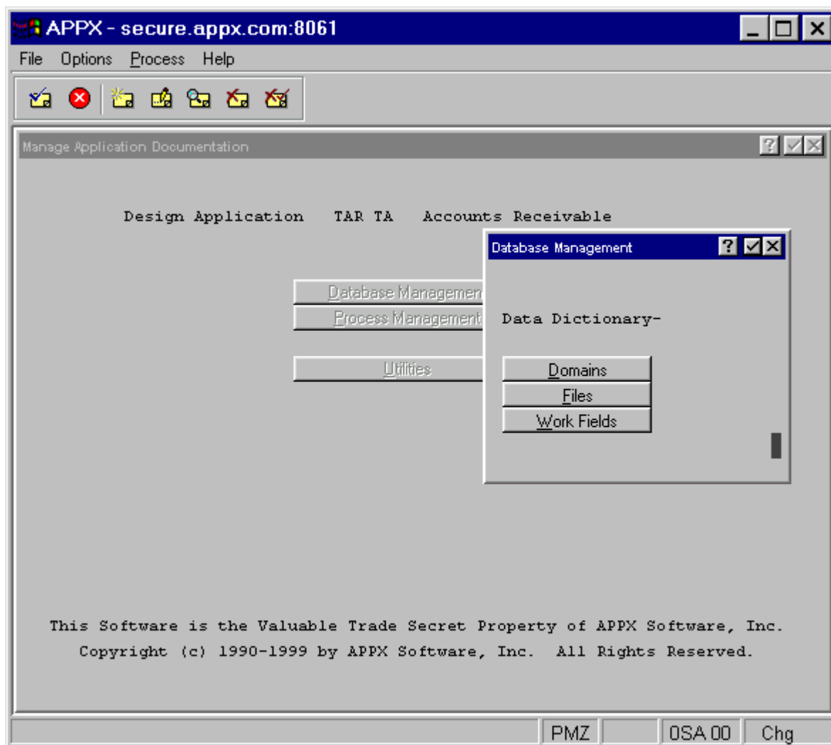
Figure 4-2. Database Documentation Management Overlay
